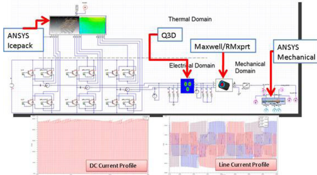
Figure 4. Multidomain simulation
