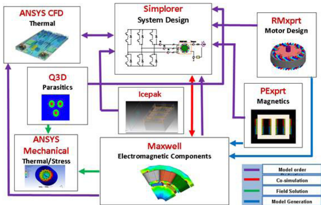
Figure 3. Systematic integrated simulation approach for motor and drives systems Simplorer® software from ANSYS is a multidomain system simulation program used for designing high-performance systems that include electrical, thermal, electromechanical, electromagnetic, controller designs, etc. Simplorer ties all these different physical analyses together to ultimately optimize the whole electric powertrain as one coherent system. This figure shows the resulting design flow.
