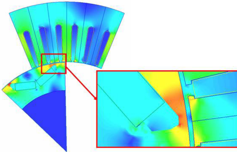
Figure 2. Finite element analysis accurately accounts for nonlinearity and local saturation of a rotor and stator. Maxwell ® electromagnetics field simulation software from ANSYS uses the finite element method to solve static, frequency-domain and time-varying electromagnetic and electric fields. A key benefit of the software is its automated solution process in which users need only specify geometry, material properties and the desired output. From this point, Maxwell automatically generates an appropriate mesh for solving the problem.
