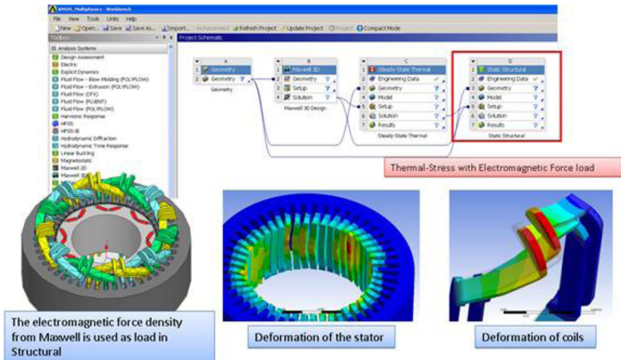
Figure 5. Typical multiphysics traction motor design problem in common simulation platform
