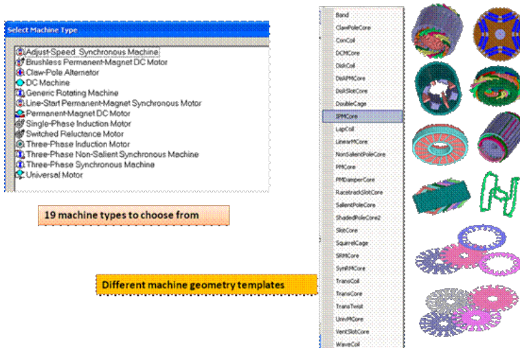
Figure 1. Types of electric machines A magnetic circuit-based motor design package — RMxprt™ from ANSYS — provides a template for 19 different types of machines. This tool quickly generates an initial design that can be imported to other higher-fidelity simulation tools.
