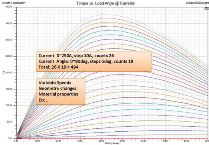
Figure 6. IPM torque output vs. load angles and currents, used to maximize output torque at different load angles and currents
