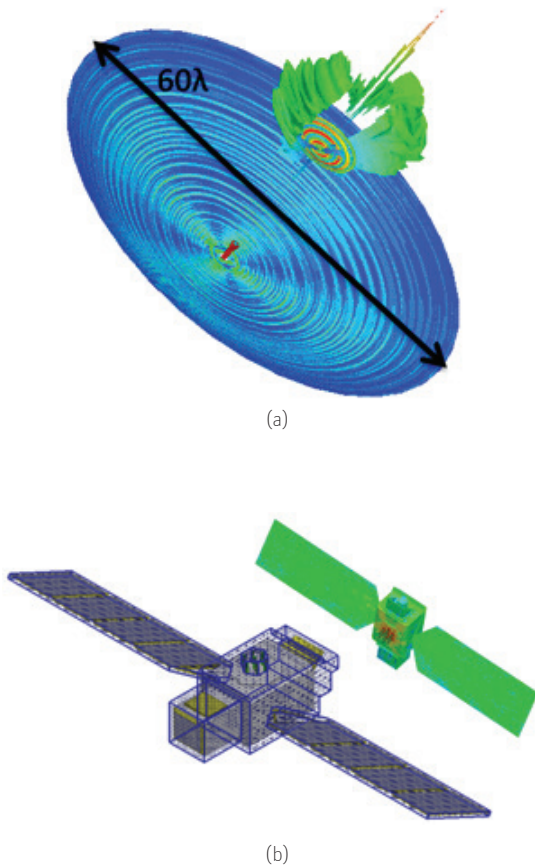
Figure 6. Hybrid simulation for two antenna structures. (a) Reflector antenna. (b) Satellite with conformal radiation boundary.
