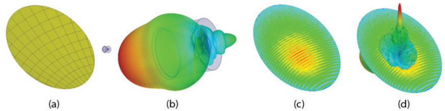
Figure 7. Physical optics solver used to simulate a reflector antenna. (a) Geometry of reflector antenna and feed horn. (b) Electric fields surrounding feed horn. (c) Surface currents on the reflector. (d) Far-field pattern superimposed on the reflector with near-field currents.
