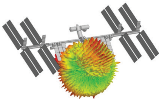
Figure 8. PO example showing antenna pattern of an antenna on International Space Station.
