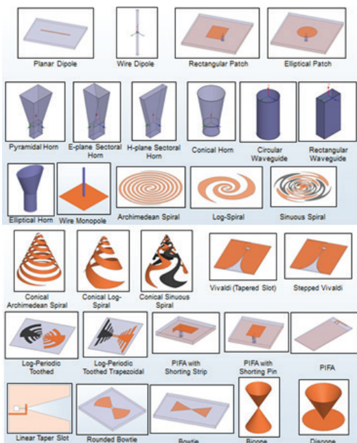
Figure 13. Available antenna types in the toolkit.
