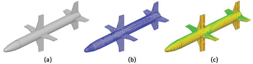
Figure 5. Integral Equations example. a) Missile Geometry. b) Surface Mesh. c) Currents on surface.
