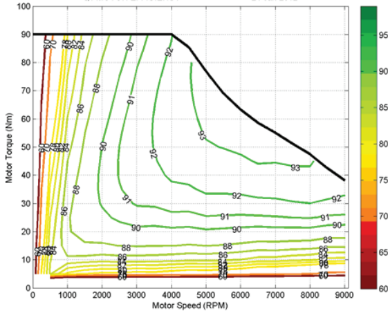
Figure 4. Experimental results of efficiency map in interior PM motor measured by Magna Electronics
