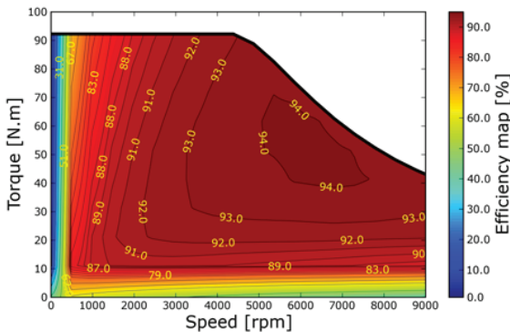
Figure 3. Simulated results of efficiency map in interior PM motor
