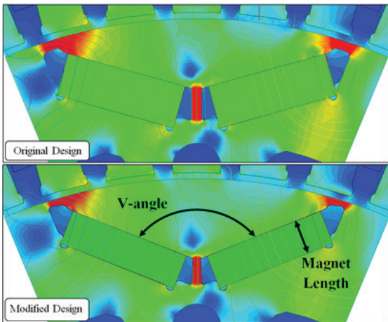
Figure 5. Original and modified designs provided by Magna Electronics. Modification included reduction of magnet length and decreased V-angle of the magnets.
